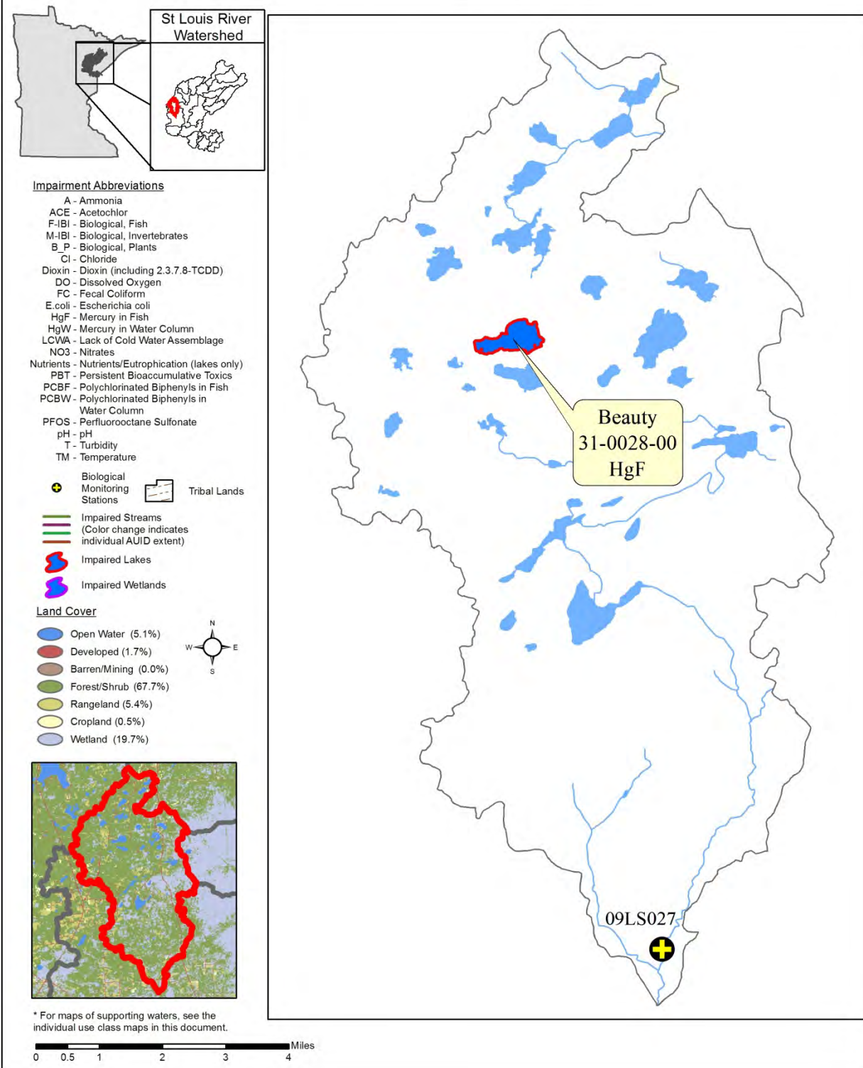
Figure 23. Currently listed impaired waters by parameter and land use in the Floodwood River Watershed Unit
