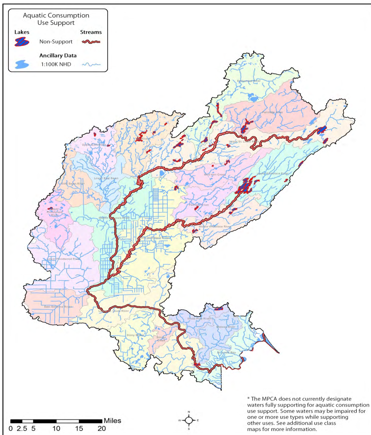
Figure 41. Aquatic consumption use support in the St. Louis River Watershed
