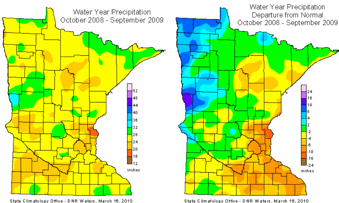
Figure 7. State-wide precipitation levels during the 2009 water year
