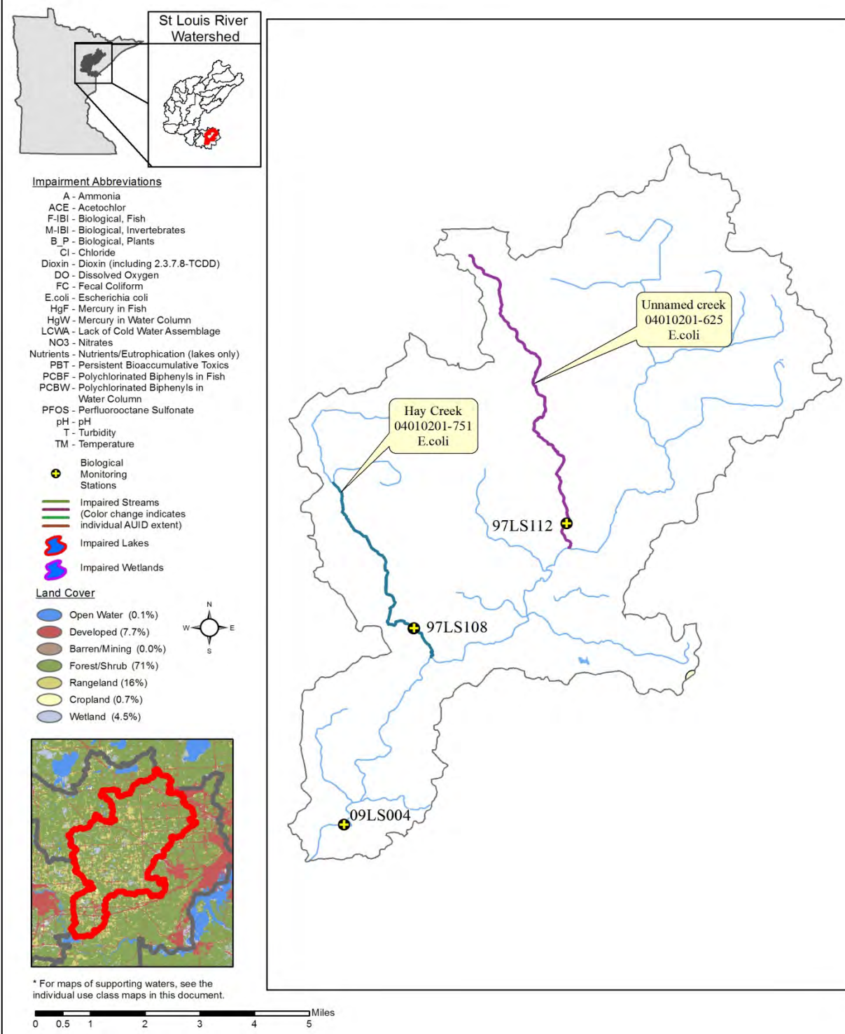
Figure 30. Currently listed impaired waters by parameter and land use in the Midway River Watershed Unit
