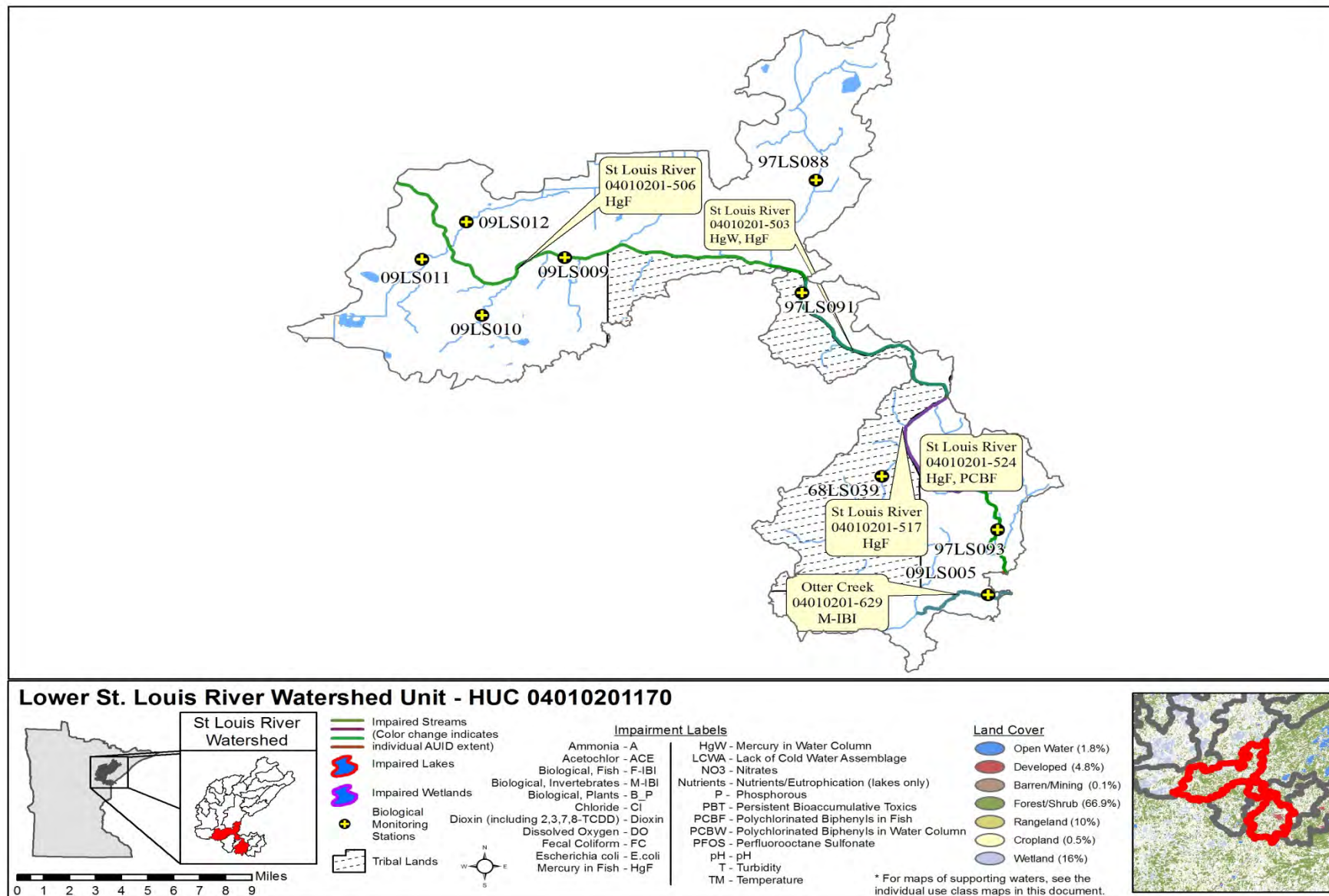
Figure 26. Currently listed impaired waters by parameter and land use in the Lower St. Louis River Watershed Unit
