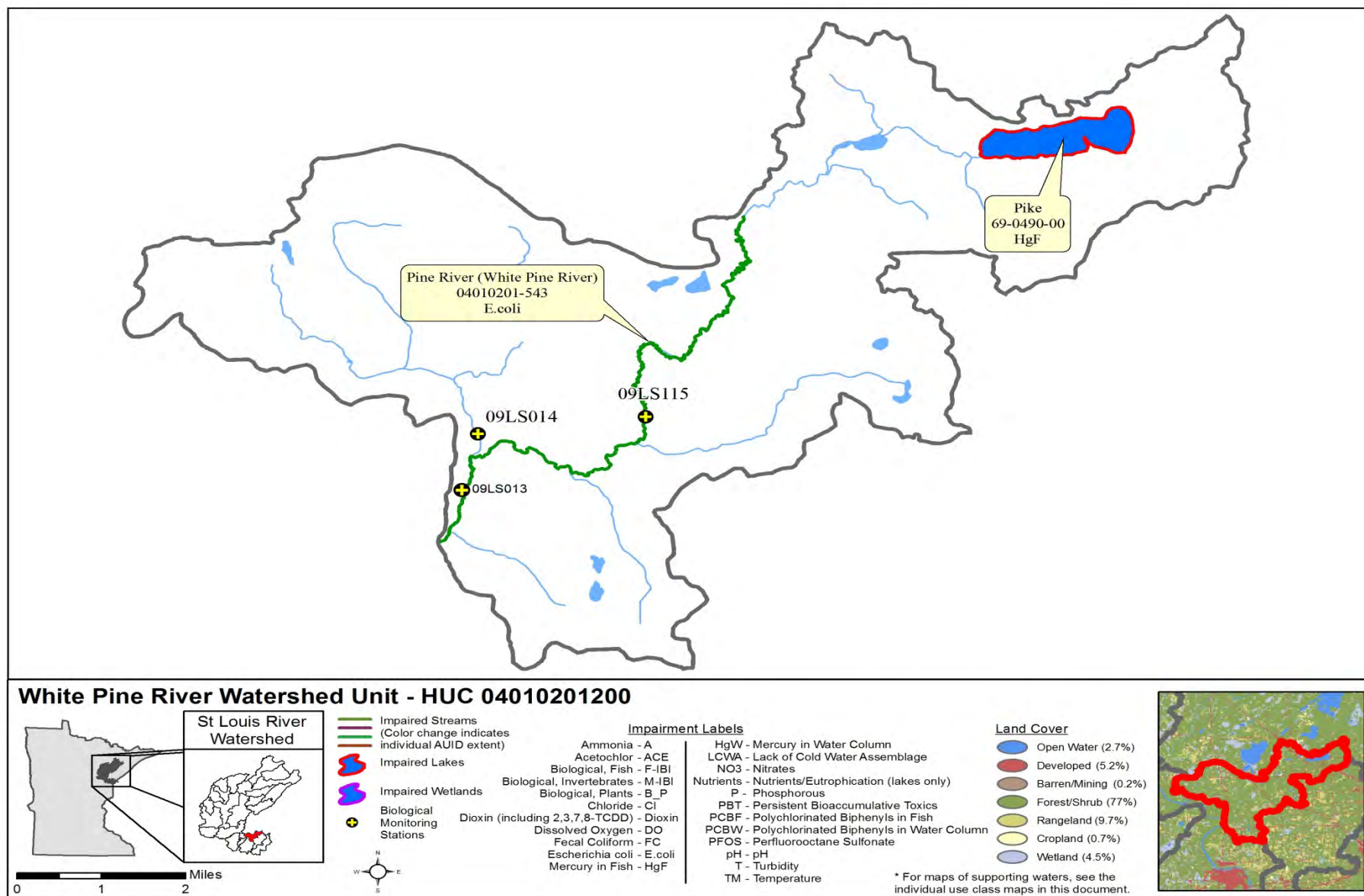
Figure 29. Currently listed impaired waters by parameter and land use in the White Pine River Watershed Unit
