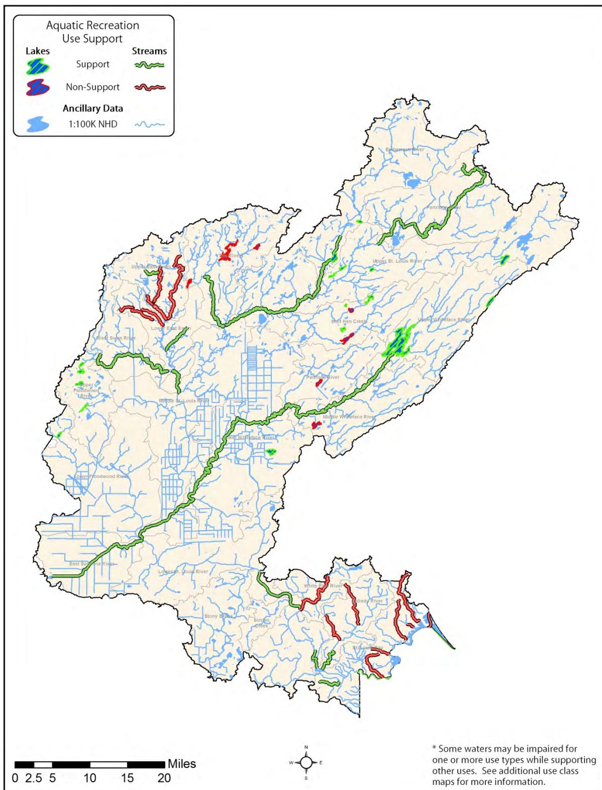
Figure 40. Aquatic recreation use support in the St. Louis River Watershed
