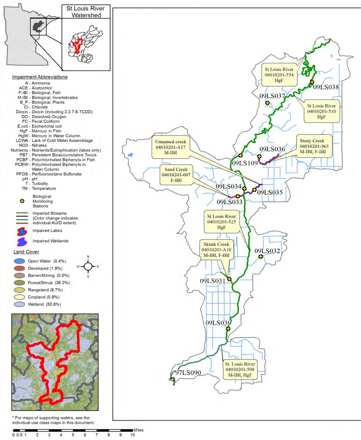
Figure 15. Currently Listed Impaired Waters by parameter and land use in the Middle St. Louis River Watershed Unit
