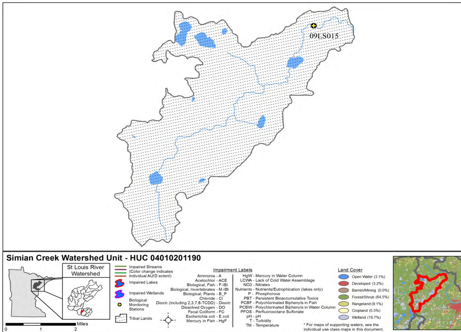
Figure 28 . Currently listed impaired waters by parameter and land use in the Simian Creek Watershed Unit
