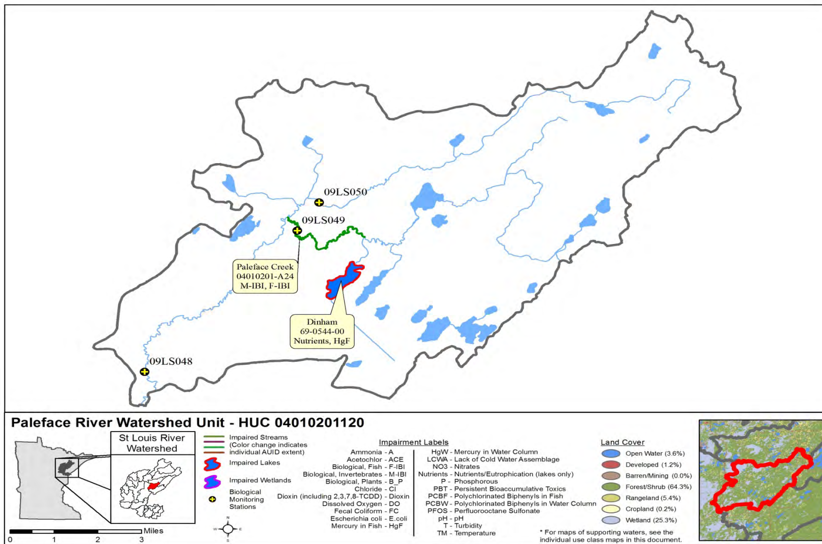
Figure 21. Currently listed impaired waters by parameter and land use in the Paleface Watershed Unit
