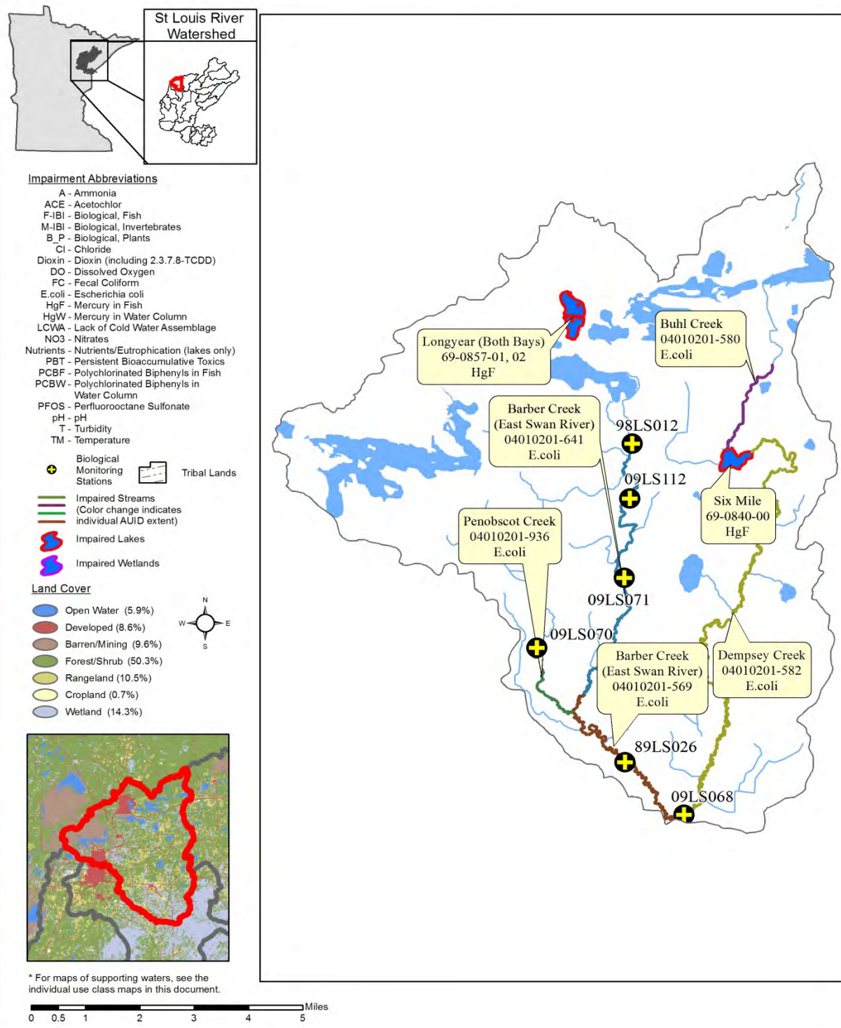
Figure 16. Currently listed impaired waters by parameter and land use in the Upper East Swan River Watershed Unit
