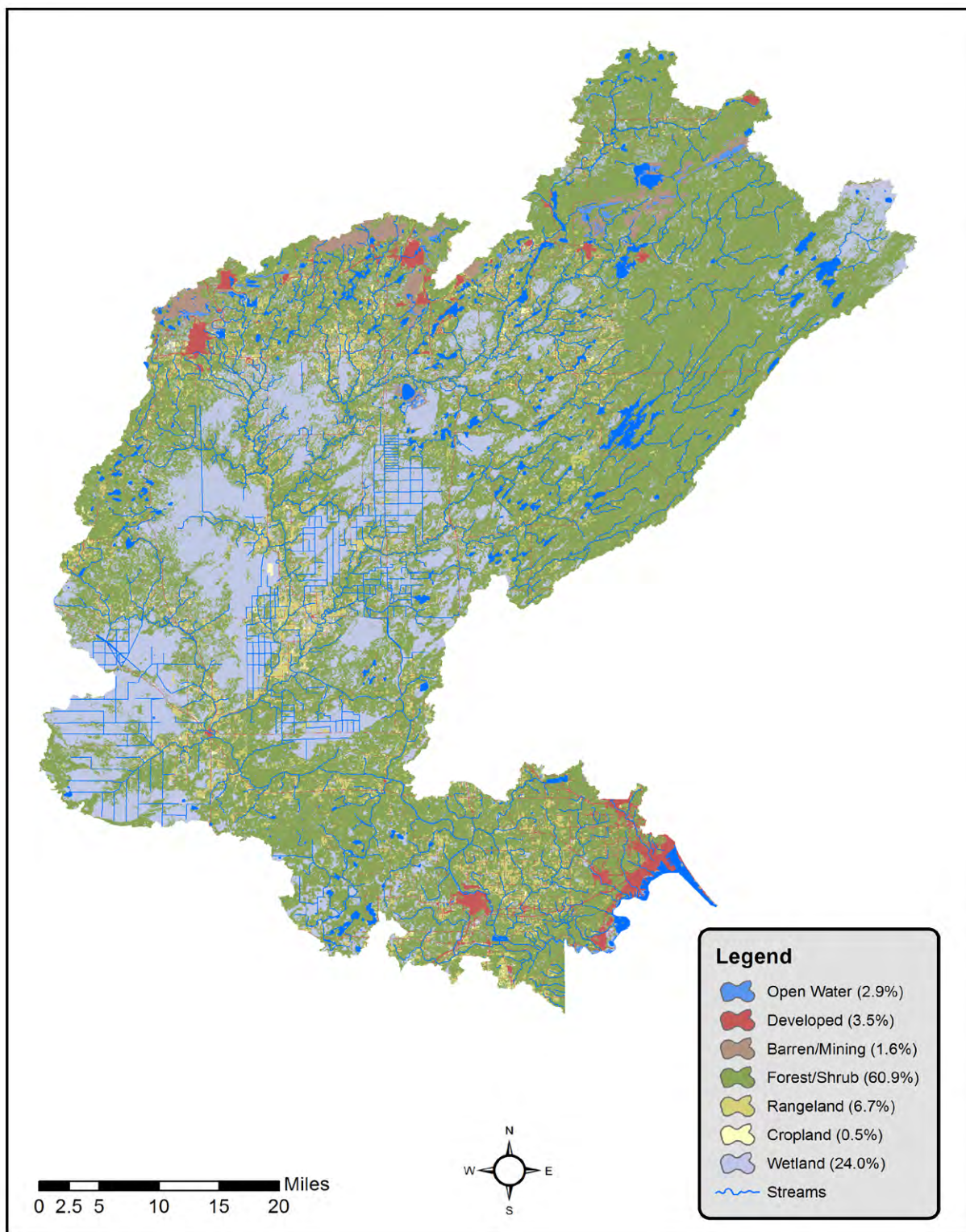
Figure 5. St. Louis Watershed 2001 land use
