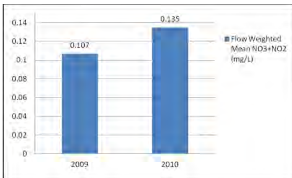
Figure 36. Nitrate + Nitrite Nitrogen (Nitrate-N) flow weighted mean concentrations for the St. Louis River
