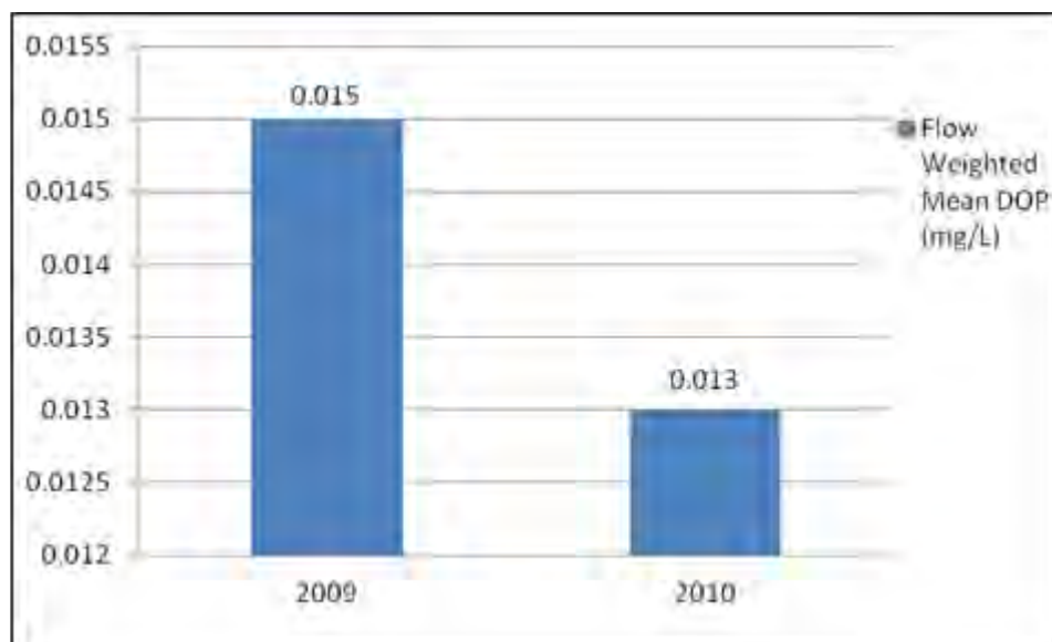
Figure 35. Dissolved Orthophosphate (DOP) flow weighted mean concentrations for the St. Louis River
