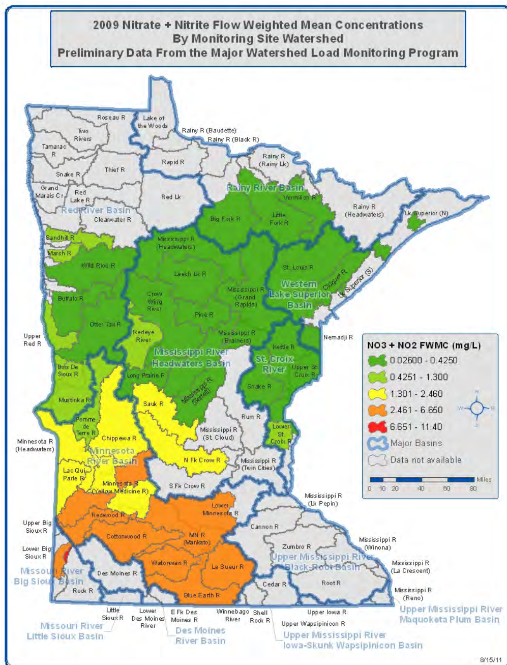
Figure 37. Nitrate - Nitrogen flow weighted mean concentrations for watershed throughout Minnesota, 2008
