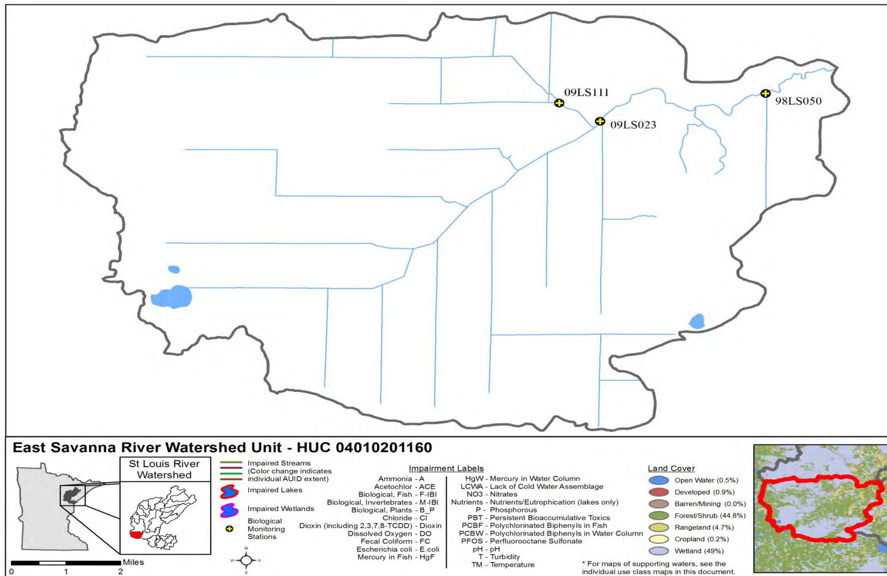
Figure 25. Currently listed impaired waters by parameter and land use in the East Savanna River Watershed Unit
