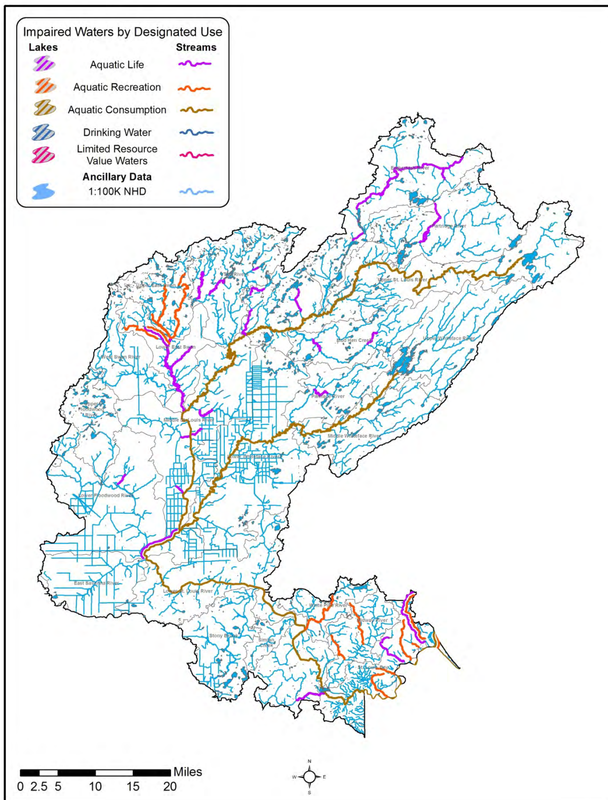
Figure 42. All impaired waters by designated use in the St. Louis River Watershed
