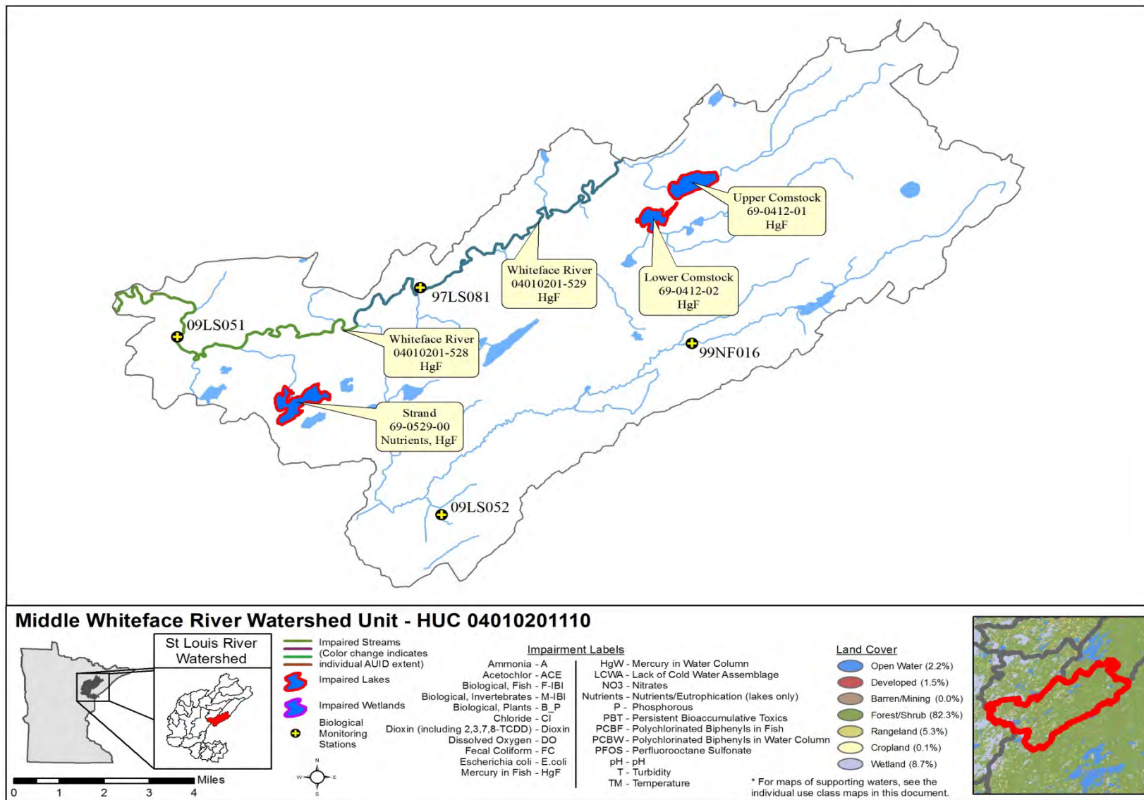
Figure 20. Currently listed impaired waters by parameter and land use in the Middle Whiteface River Watershed Unit
