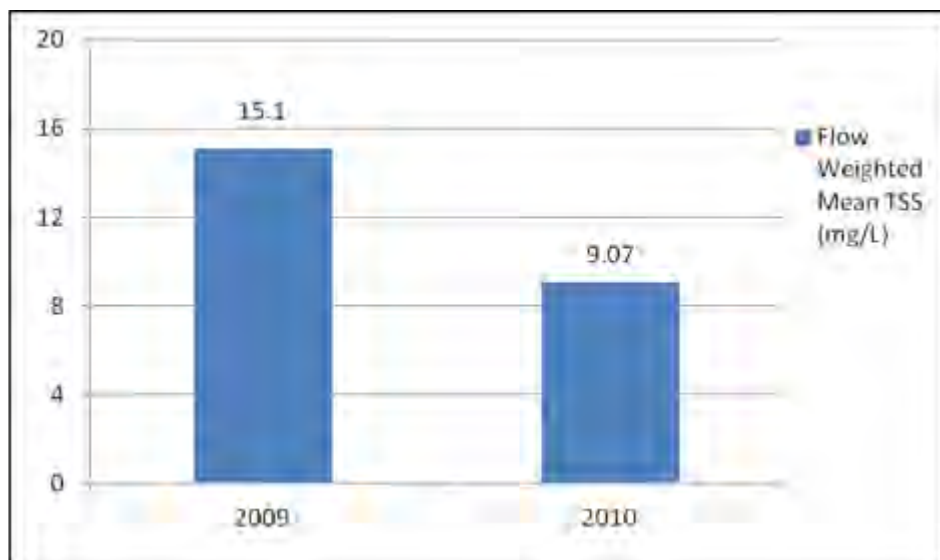
Figure 33. Total Suspended Solids (TSS) flow weighted mean concentrations for the St. Louis River
