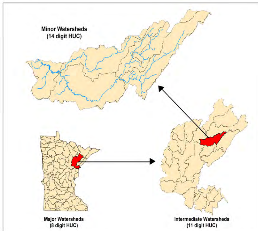
Figure 2. The intensive watershed monitoring design
