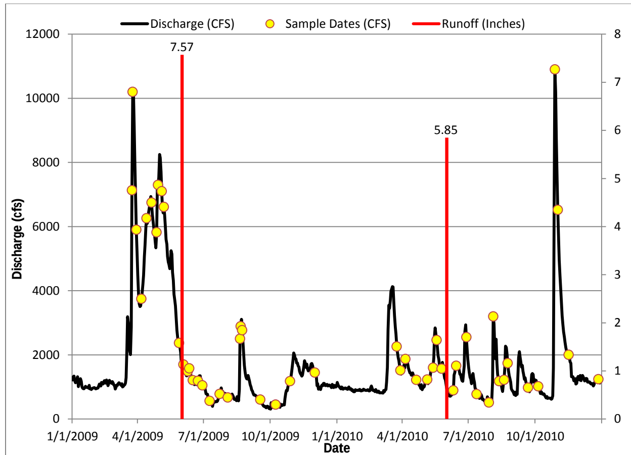
Figure 32. Hydrograph for the St. Louis River 2009-2010
