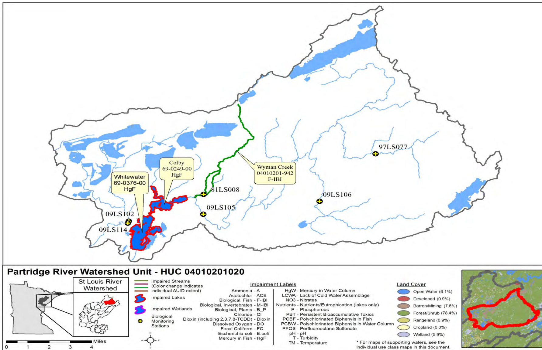
Figure 11. Currently Listed Impaired Waters by parameter and land use in the Partridge River Watershed Unit
