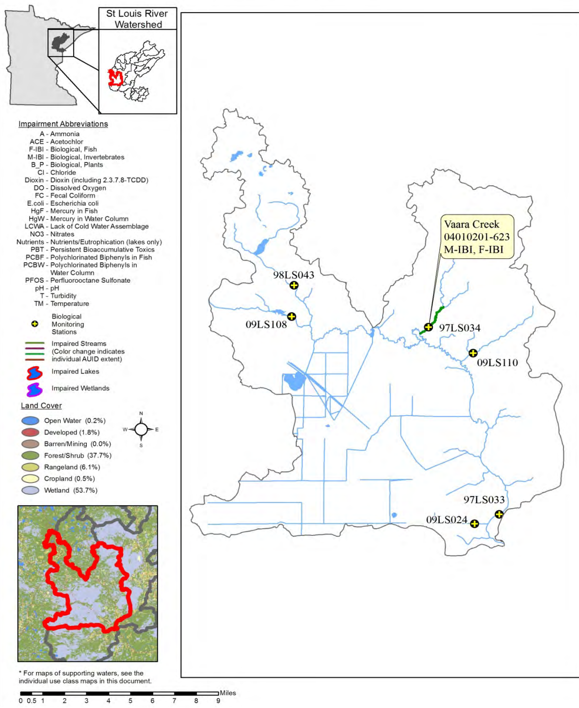
Figure 24. Currently listed impaired waters by parameter and land use in the Lower Floodwood River Watershed Unit
