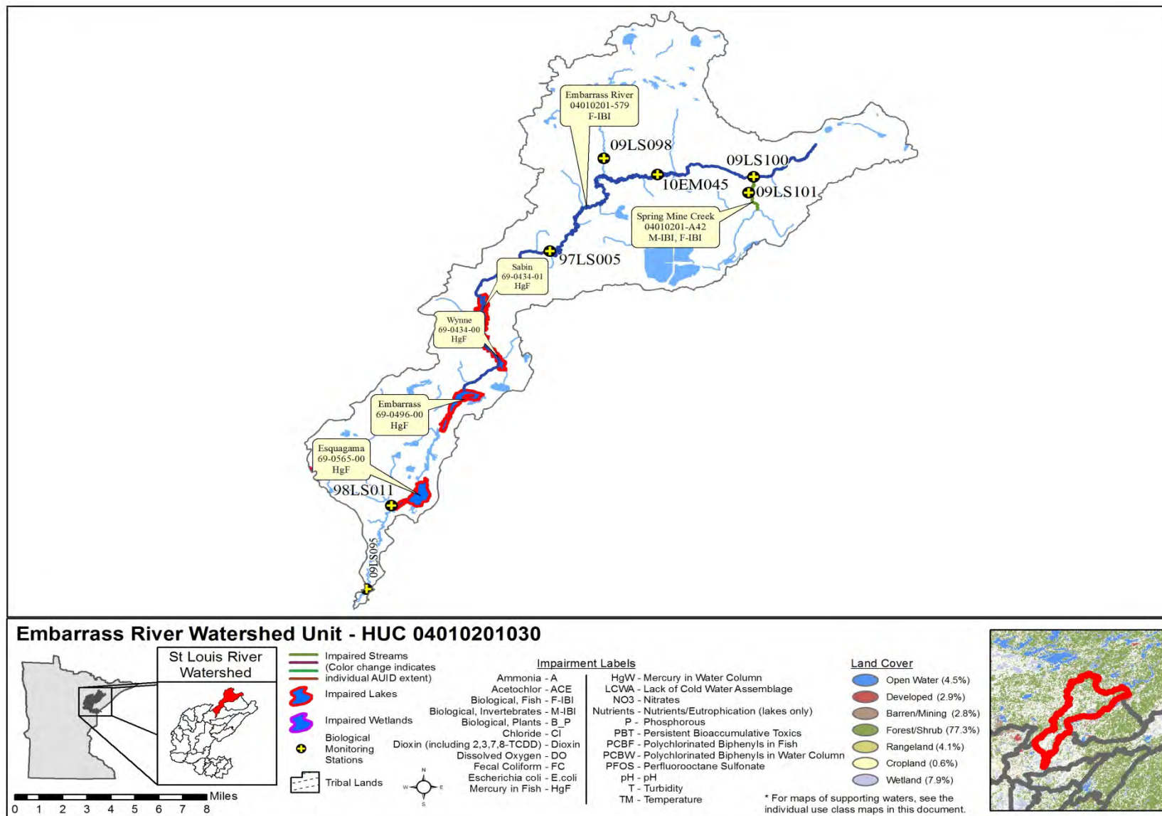
Figure 12. Currently Listed Impaired Waters by parameter and land use in the Embarrass River Watershed Unit
