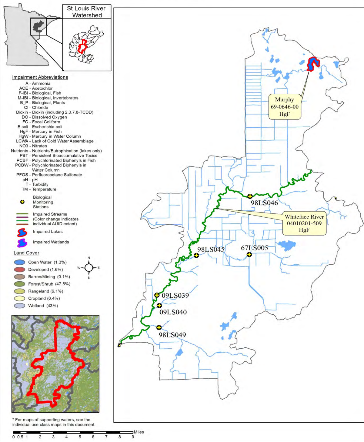
Figure 22. Currently listed impaired waters by parameter and land use in the Lower Whiteface River Watershed Unit
