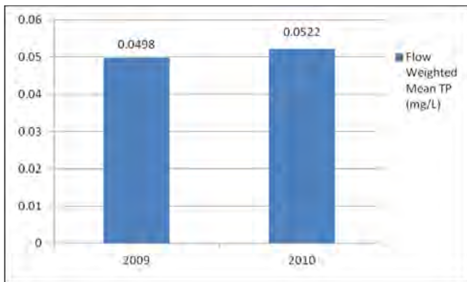
Figure 34. Total Phosphorus (TP) flow weighted mean concentrations for the St. Louis River
