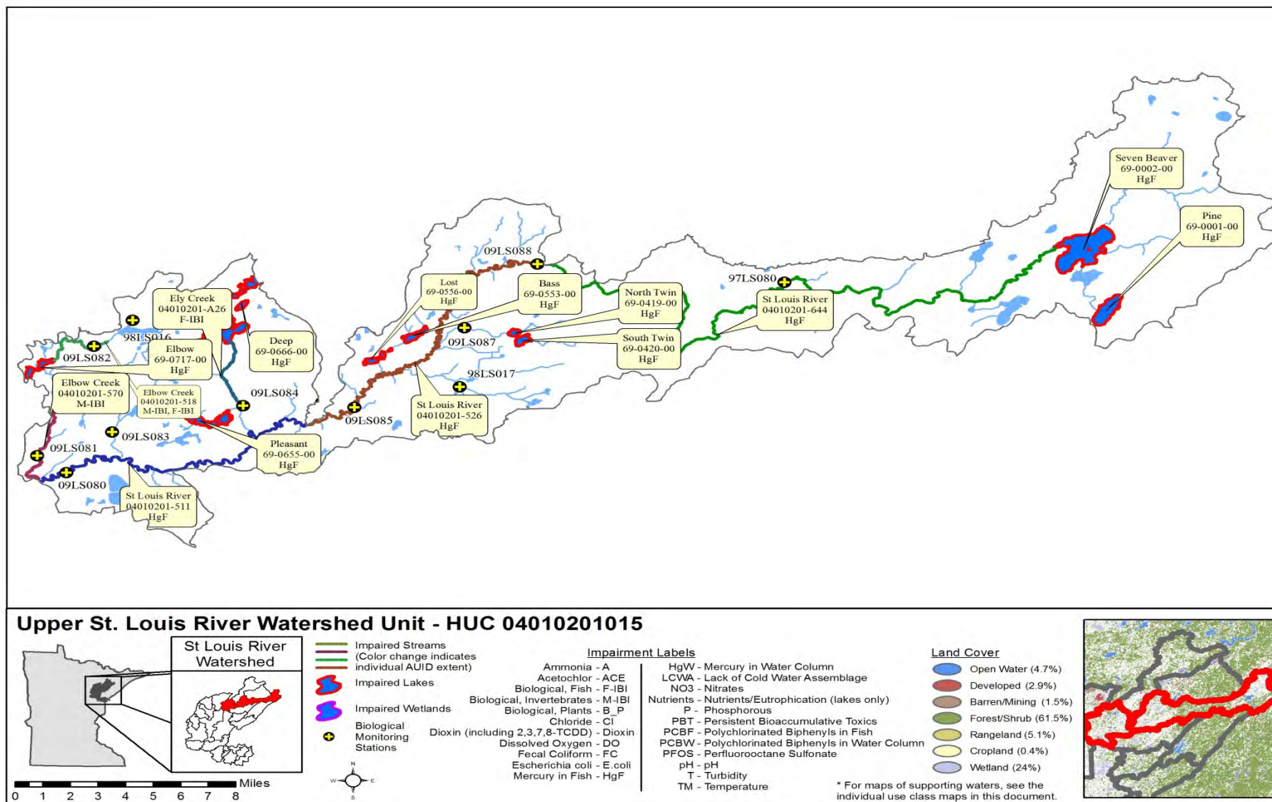
Figure 10. Currently Listed Impaired Waters by parameter and land use in the St. Louis River Watershed Unit
