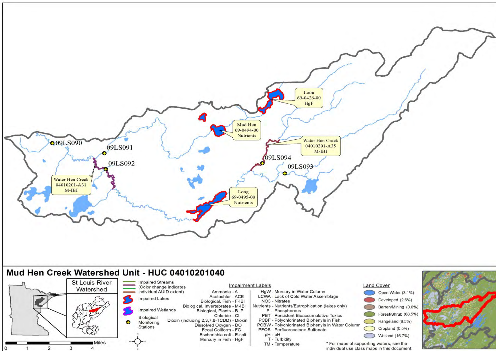
Figure 13. Currently Listed Impaired Waters by parameter and land use in the Mud Hen Creek Watershed Unit
