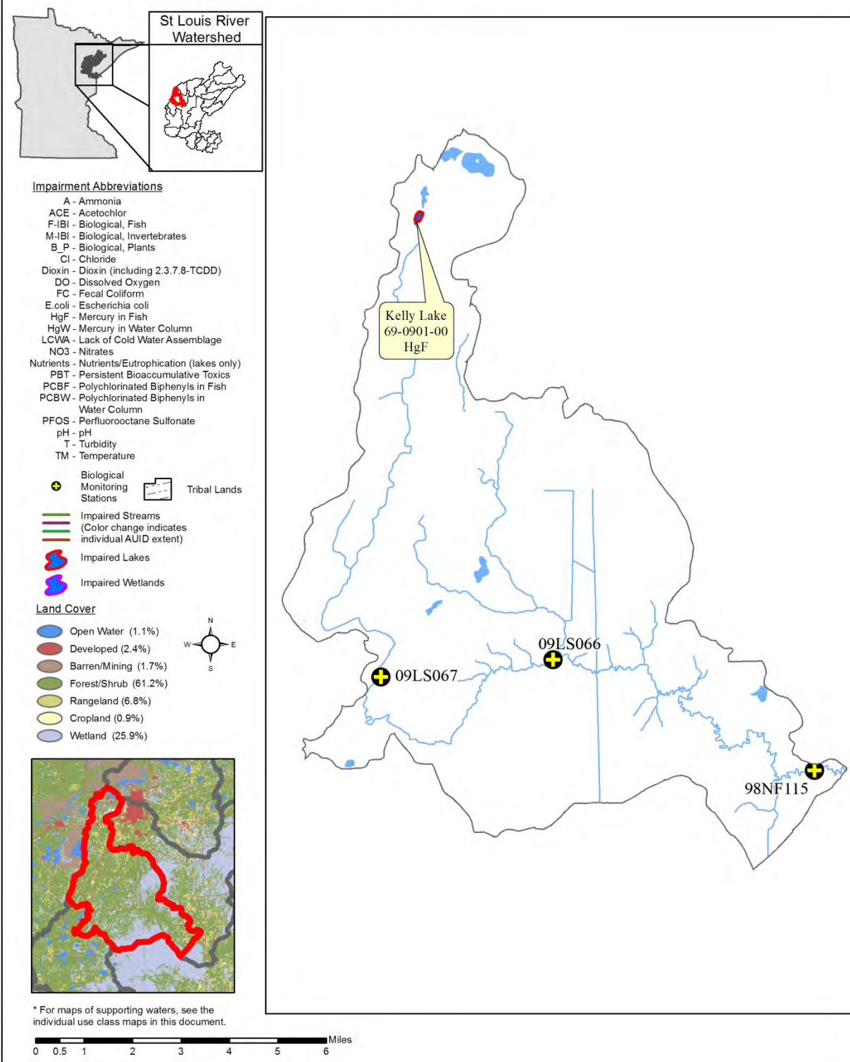
Figure 17. Currently Listed Impaired Waters by parameter and land use in the West Swan River Watershed Unit
